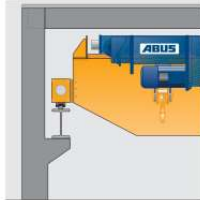
Stooped down configuration Version 2
